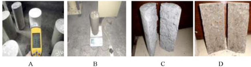
Figure 4 Temperature measurement of cylinder concrete with organic cement (A), Weight measurement of cylinder concrete with organic cement (B), Concrete cylinder with organic cement of tensile test result (C), Concrete cylinder with portland cement of tensile test result (D)
